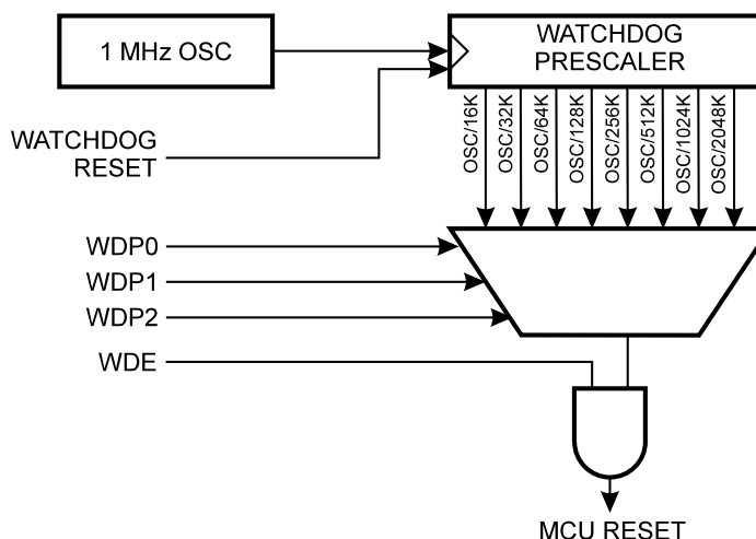
Figure 20. Watchdog Timer
